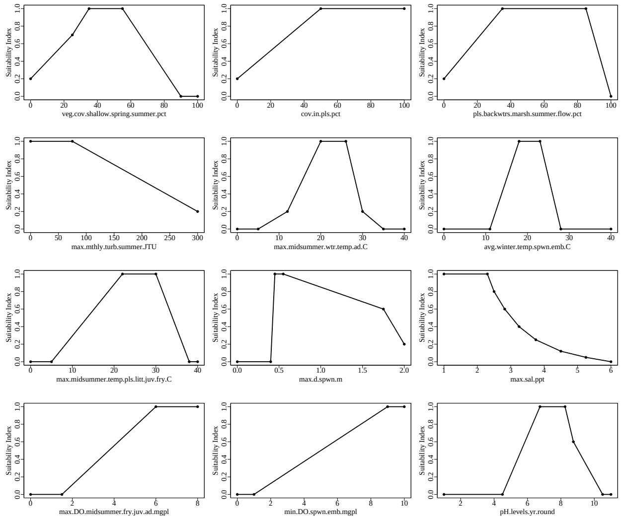
Figure 1. Suitability index graphs for variables included in the commoncarpRivSal model in ecorest.
